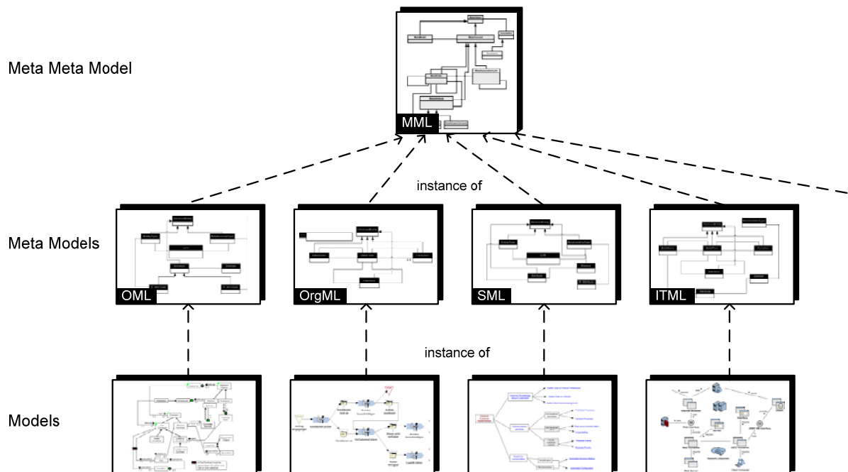
Figure 16: The MEMO language layers
