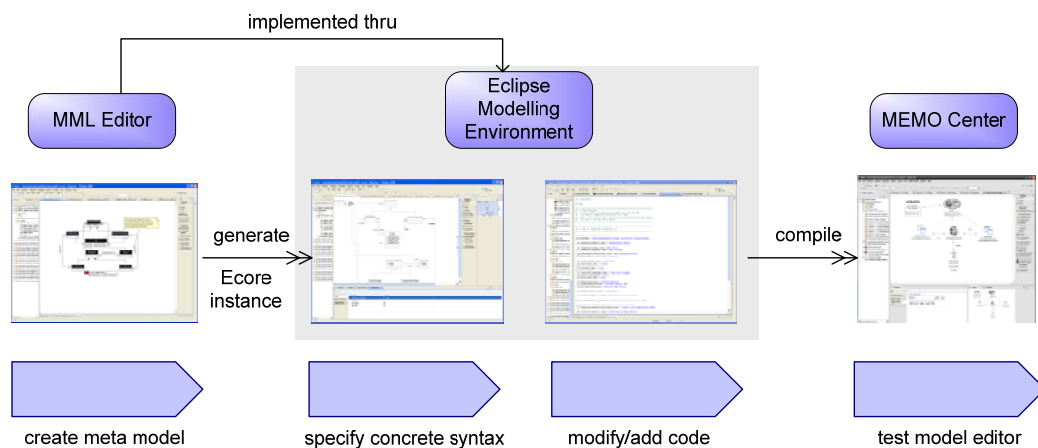
Figure 19: Simplified workflow for developing additional model editors within MEMO Center
