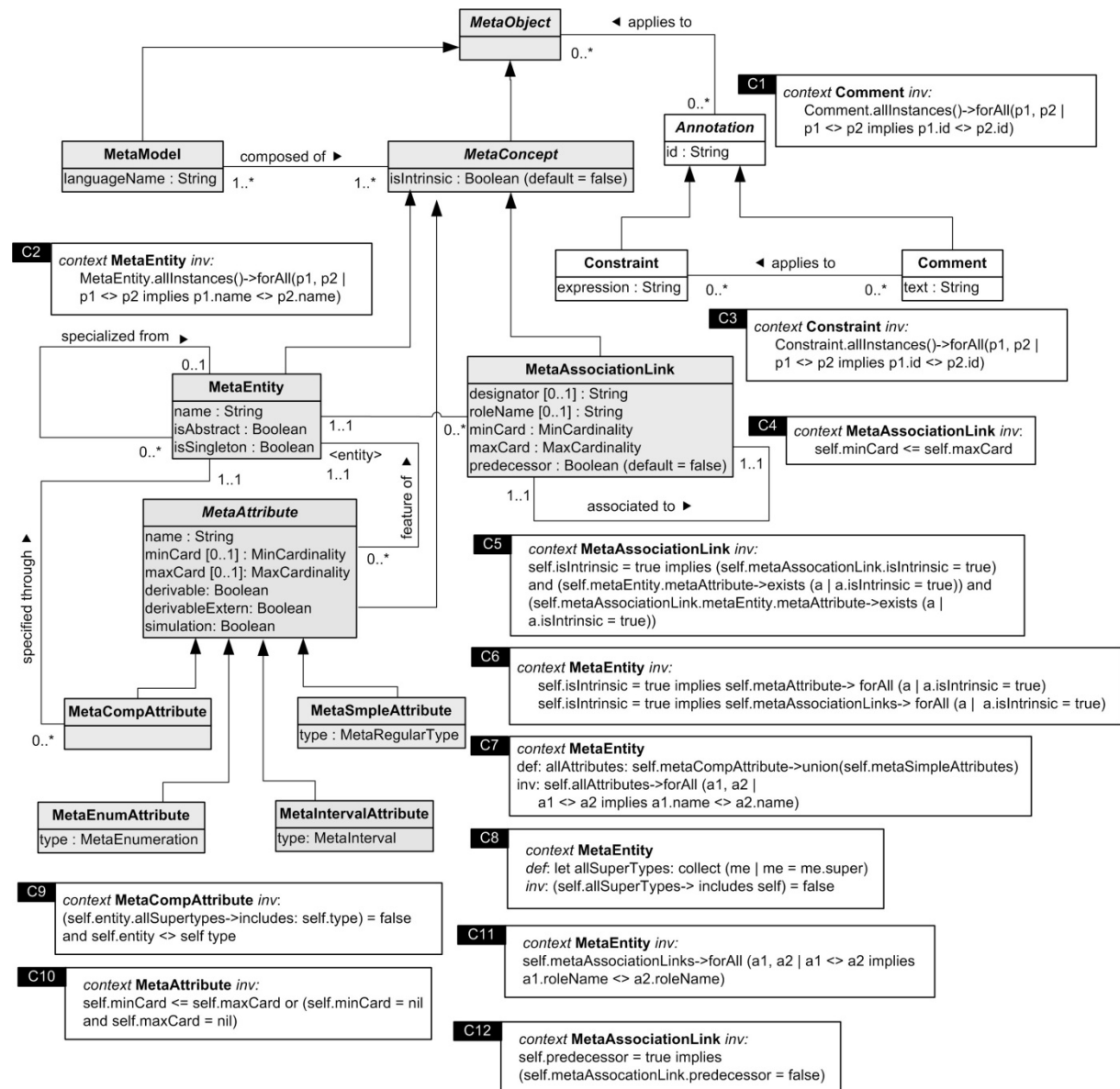
Figure 10: The MEMO meta meta model
