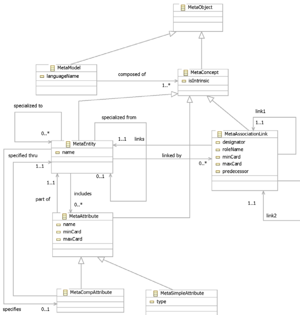
Figure 18: The MEMO meta meta model as an Ecore instance
