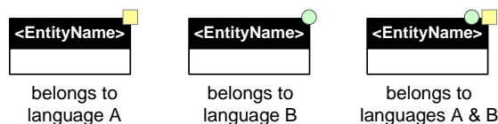
Figure 12: Options to mark the elements of a meta model as belonging to a particular language
