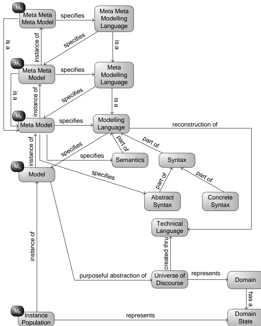
Figure 1: Semantic net of key terms and corresponding levels of abstraction
