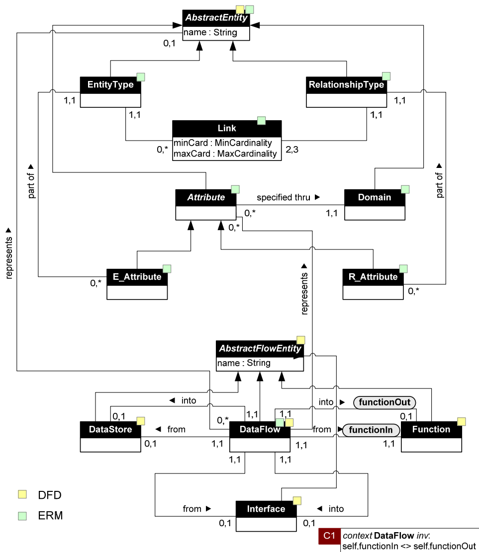
Figure 14: Differentiating two meta models through specific symbols
