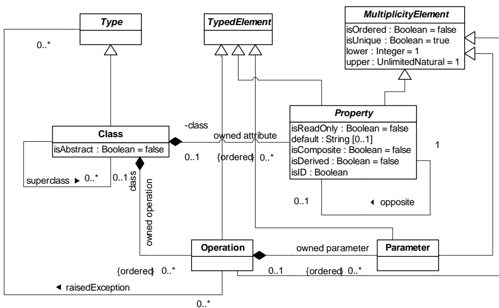
Figure 3: Revised version of EMOF
