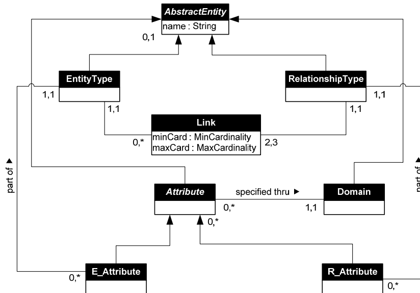
Figure 13: A meta model of the ERM
