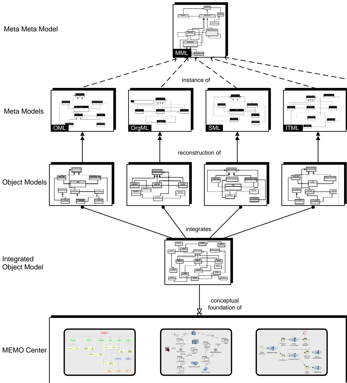
Figure 17: The MEMO language architecture and corresponding conceptual foundation for modelling tools
