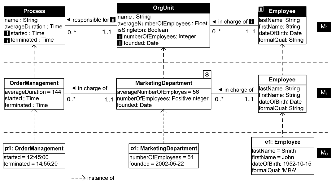
Figure 15: The use of intrinsic features
